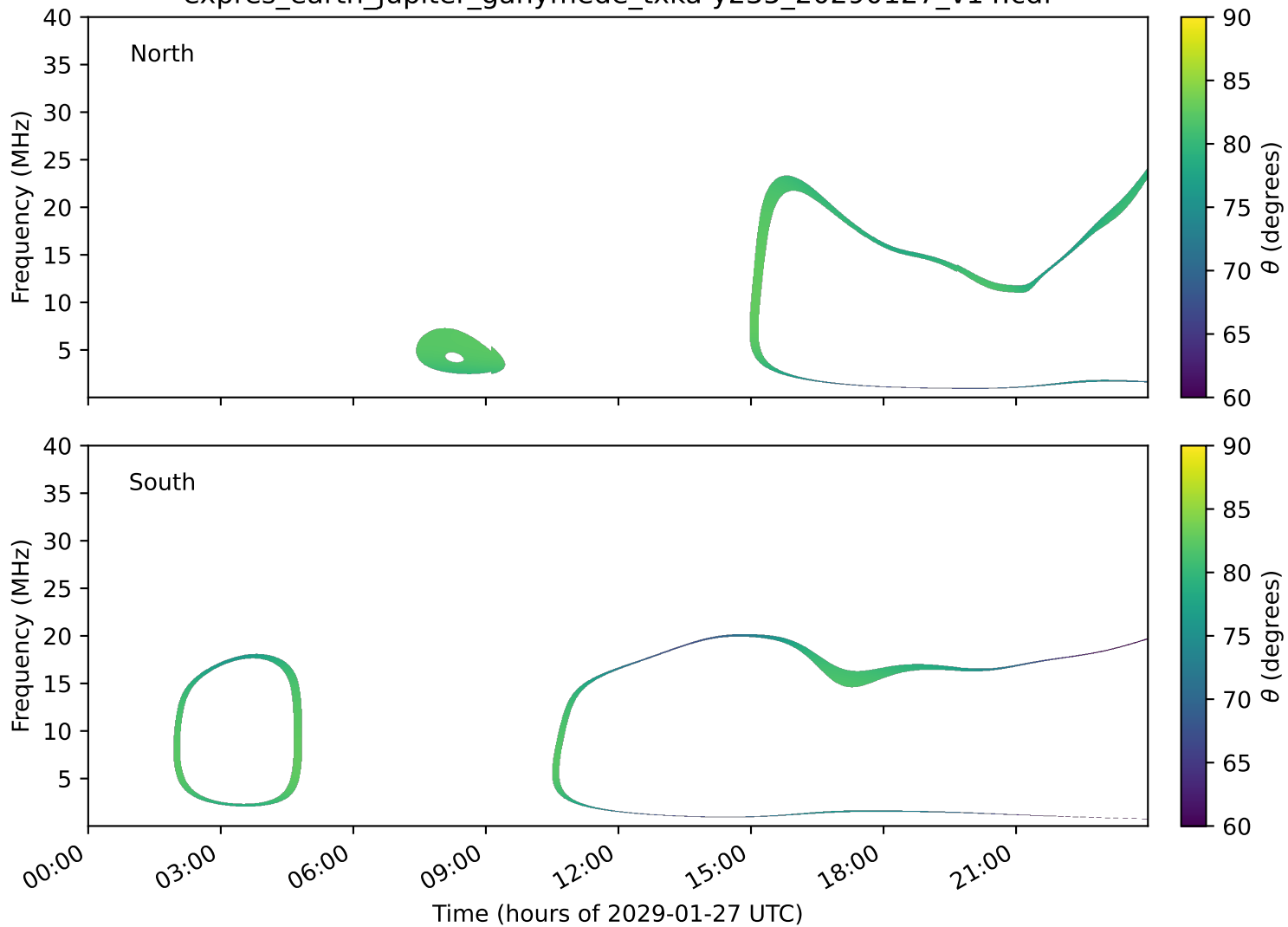
expres_earth_jupiter_ganymede_txka-y235_20290127_v14.cdf
