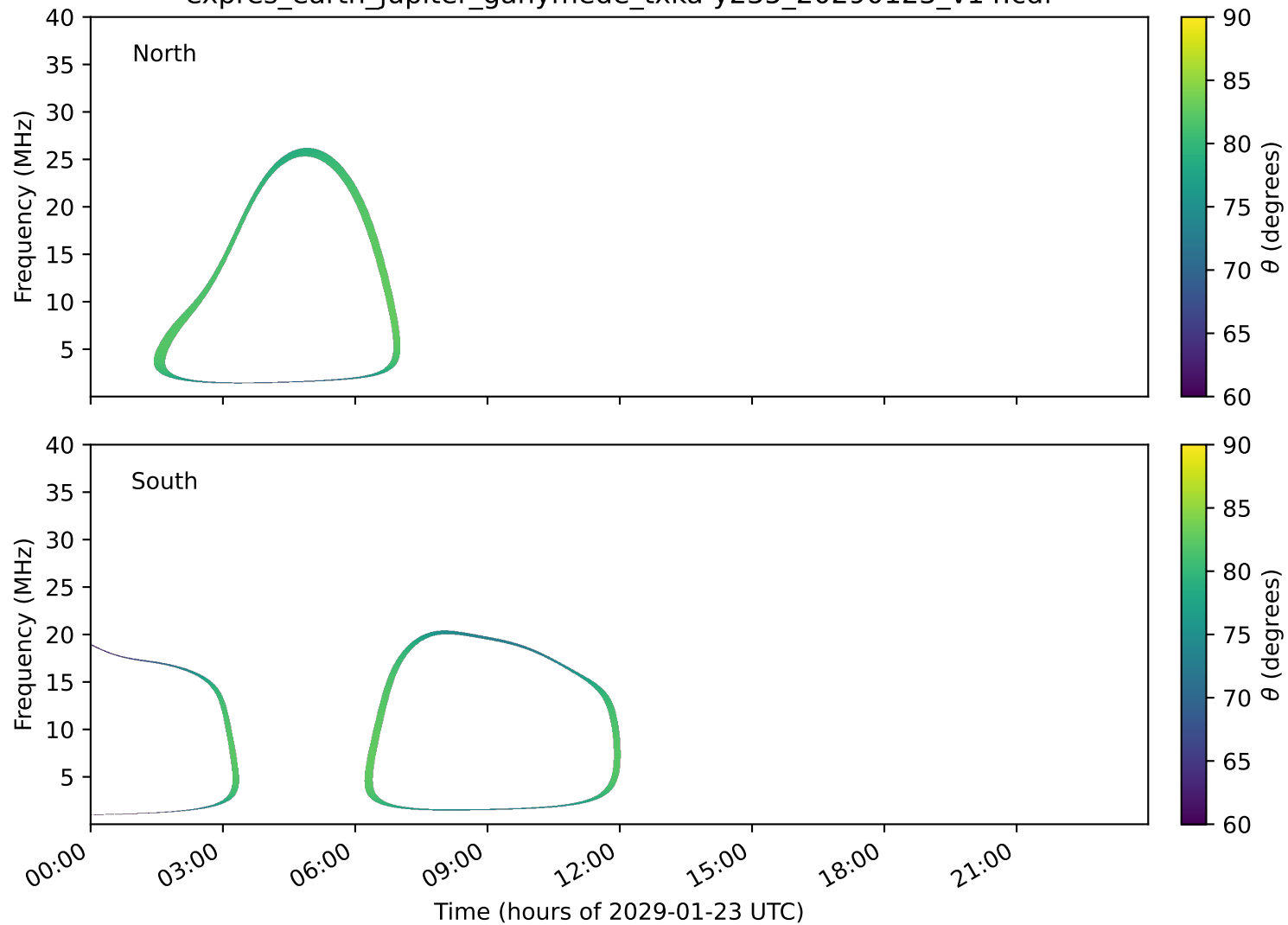
expres_earth_jupiter_ganymede_txka-y235_20290123_v14.cdf
