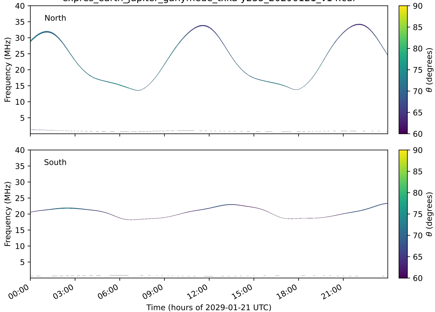
expres_earth_jupiter_ganymede_txka-y235_20290121_v14.cdf
