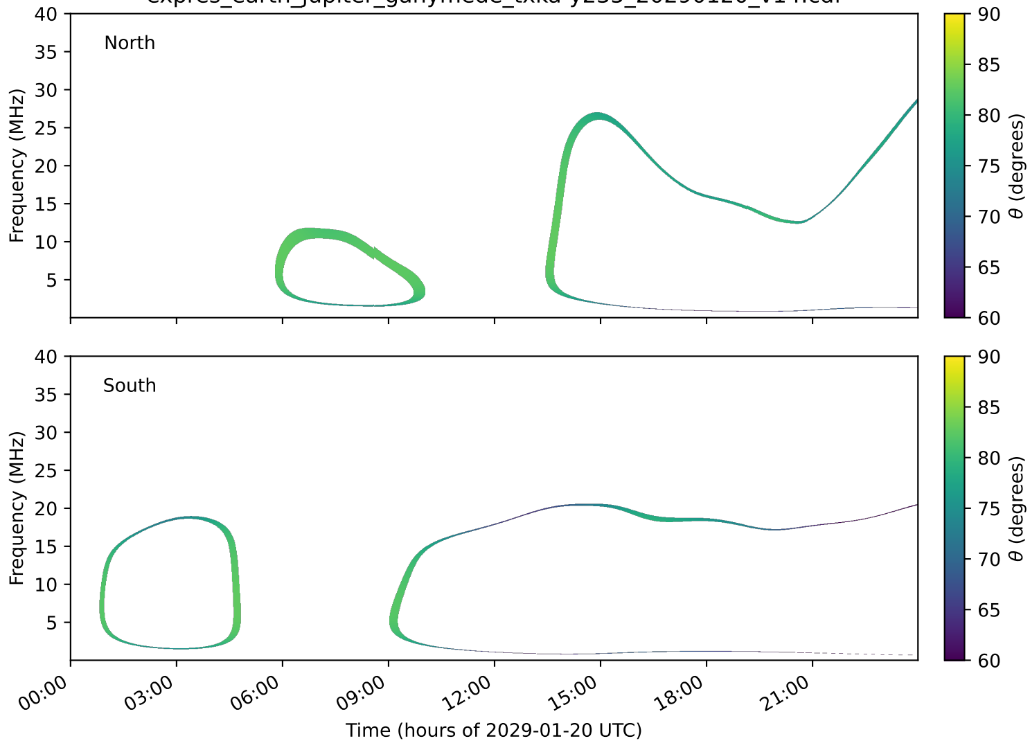
expres_earth_jupiter_ganymede_txka-y235_20290120_v14.cdf
