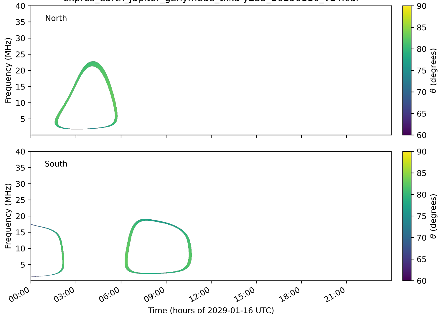
expres_earth_jupiter_ganymede_txka-y235_20290116_v14.cdf
