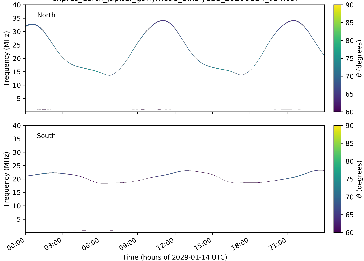
expres_earth_jupiter_ganymede_txka-y235_20290114_v14.cdf
