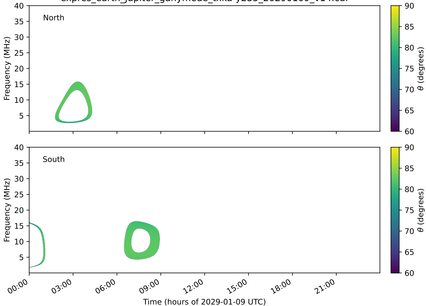
expres_earth_jupiter_ganymede_txka-y235_20290109_v14.cdf
