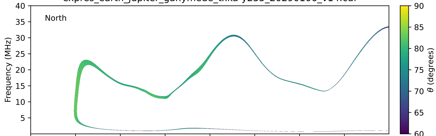
expres_earth_jupiter_ganymede_txka-y235_20290106_v14.cdf
