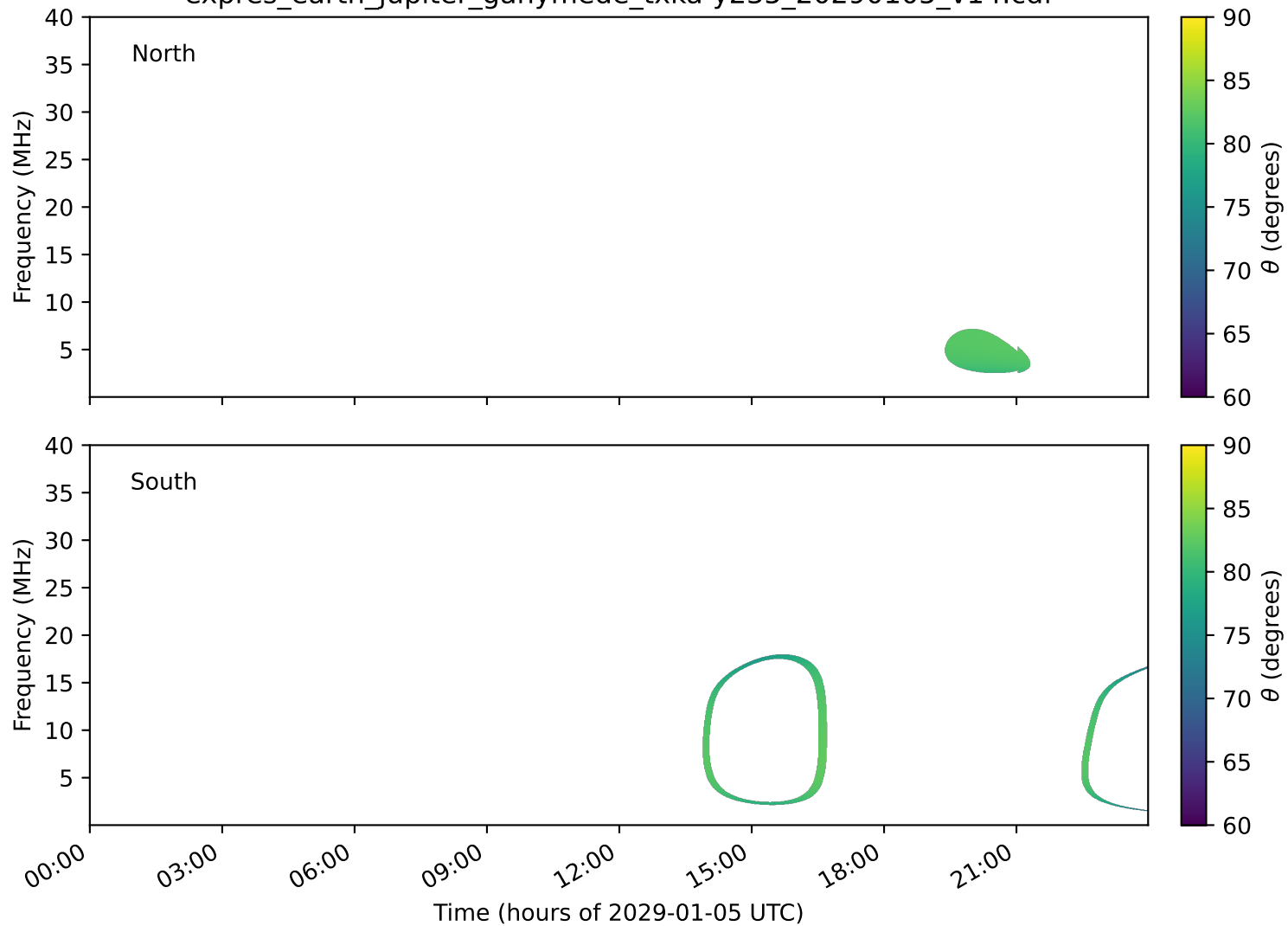
expres_earth_jupiter_ganymede_txka-y235_20290105_v14.cdf
