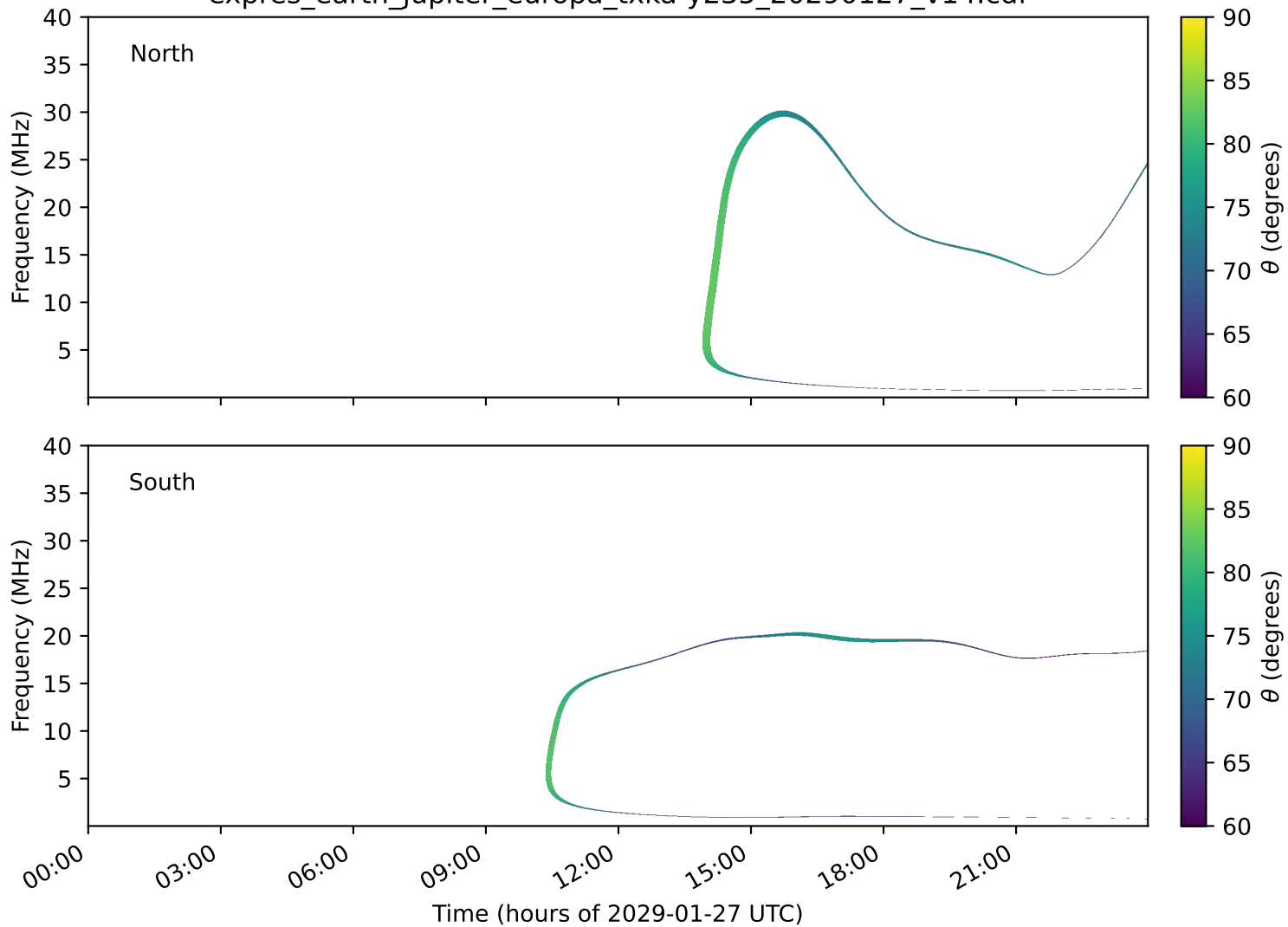
expres_earth_jupiter_europa_txka-y235_20290127_v14.cdf
