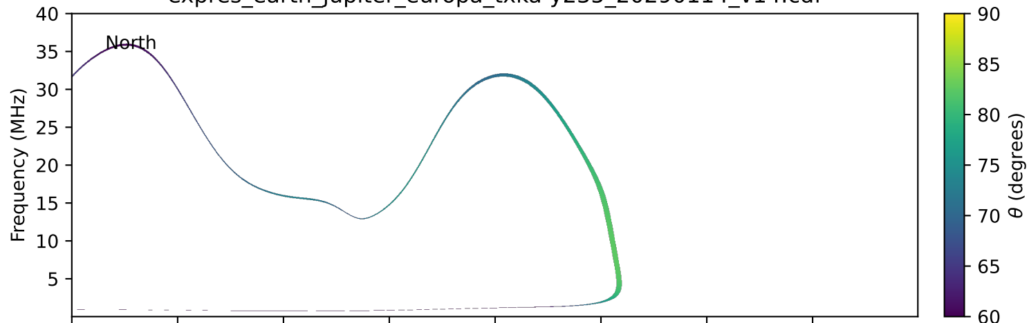
expres_earth_jupiter_europa_txka-y235_20290114_v14.cdf
