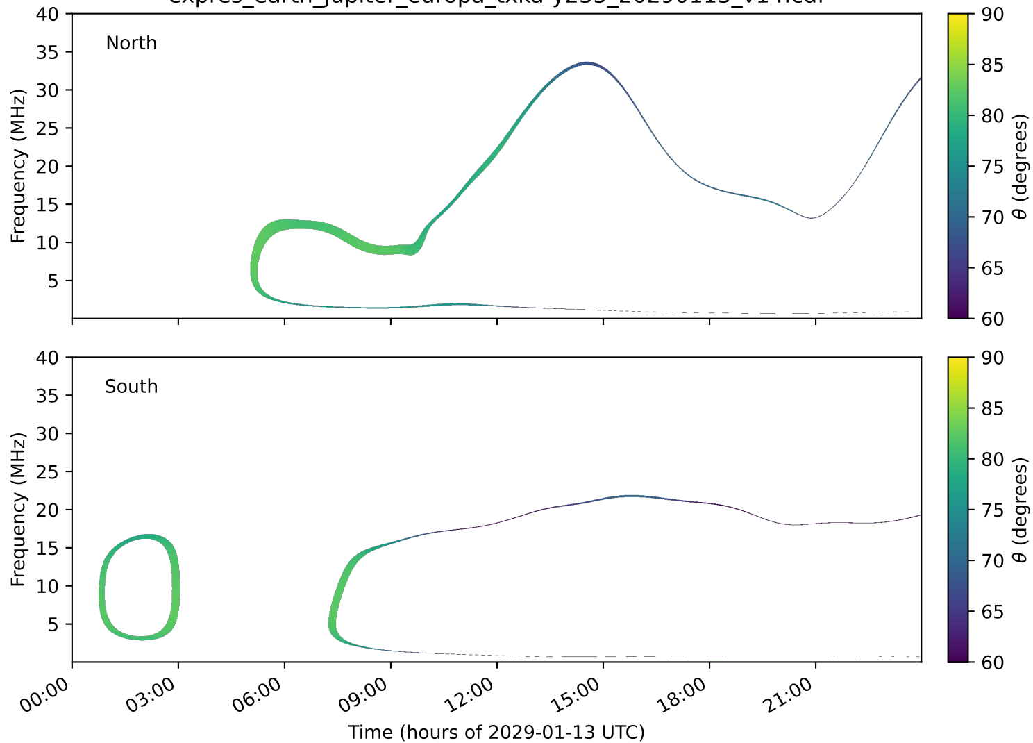
expres_earth_jupiter_europa_txka-y235_20290113_v14.cdf
