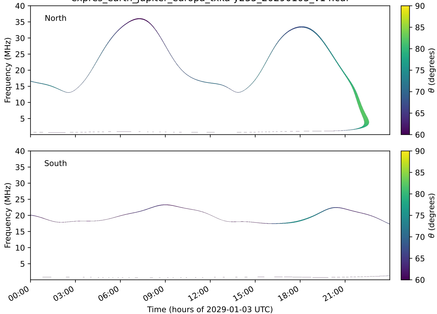
expres_earth_jupiter_europa_txka-y235_20290103_v14.cdf
