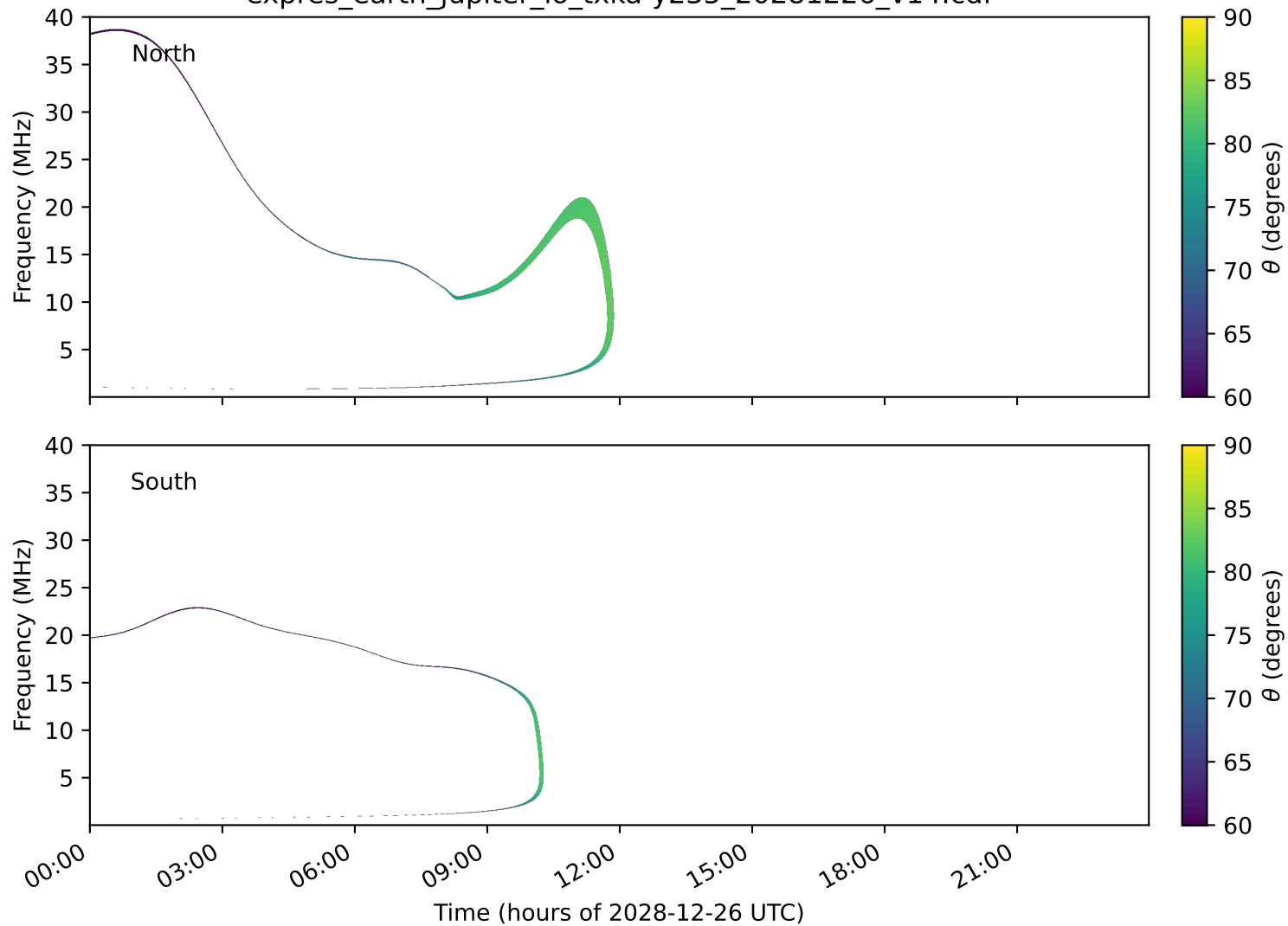
expres_earth_jupiter_io_txka-y235_20281226_v14.cdf
