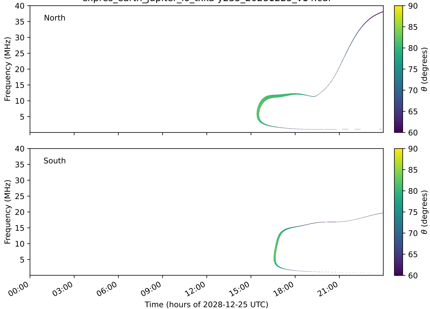
expres_earth_jupiter_io_txka-y235_20281225_v14.cdf
