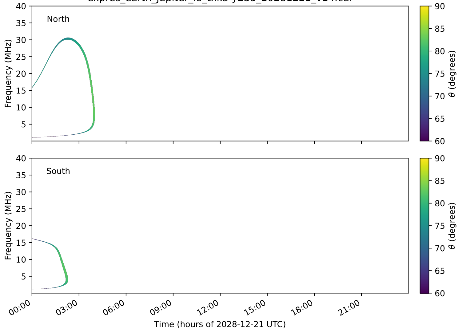
expres_earth_jupiter_io_txka-y235_20281221_v14.cdf
