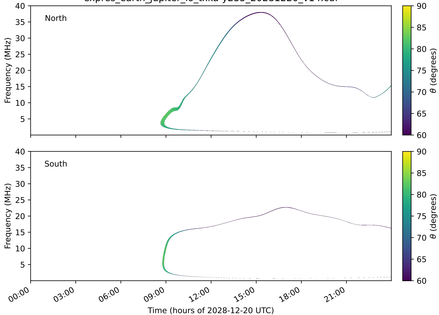
expres_earth_jupiter_io_txka-y235_20281220_v14.cdf
