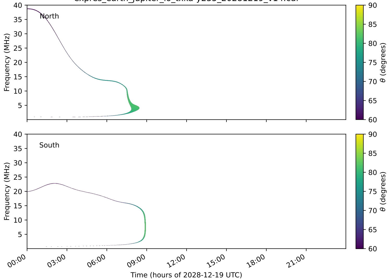
expres_earth_jupiter_io_txka-y235_20281219_v14.cdf
