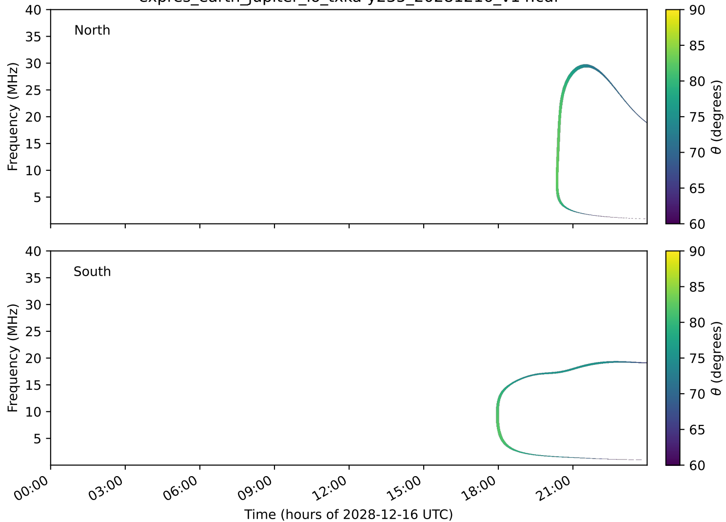
expres_earth_jupiter_io_txka-y235_20281216_v14.cdf
