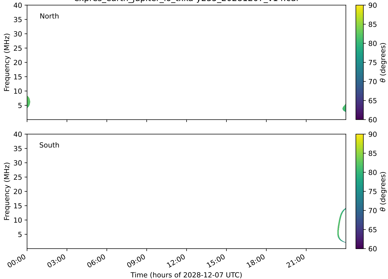
expres_earth_jupiter_io_txka-y235_20281207_v14.cdf
