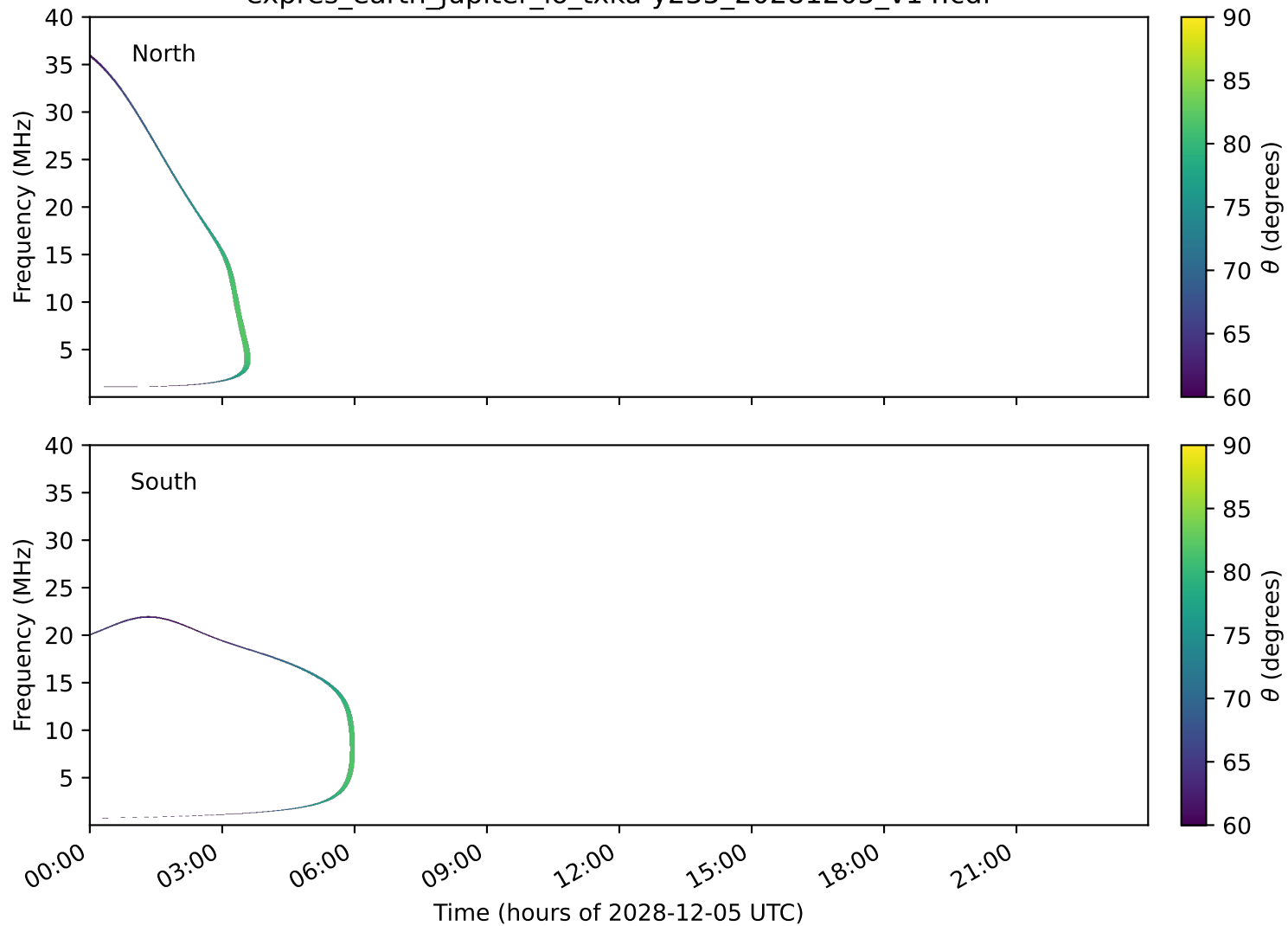
expres_earth_jupiter_io_txka-y235_20281205_v14.cdf
