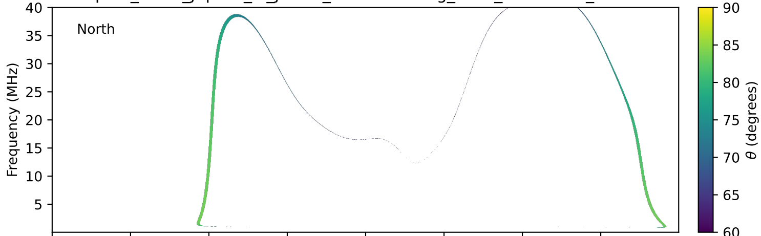
expres_earth_jupiter_io_jrm33_lossc-wid1deg_3kev_20281229_v11.cdf
