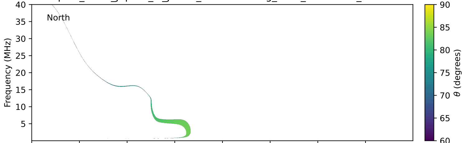
expres_earth_jupiter_io_jrm33_lossc-wid1deg_3kev_20281219_v11.cdf
