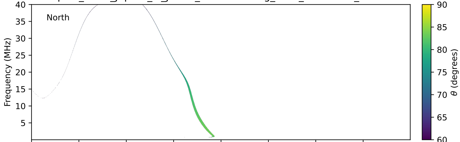
expres_earth_jupiter_io_jrm33_lossc-wid1deg_3kev_20281201_v11.cdf
