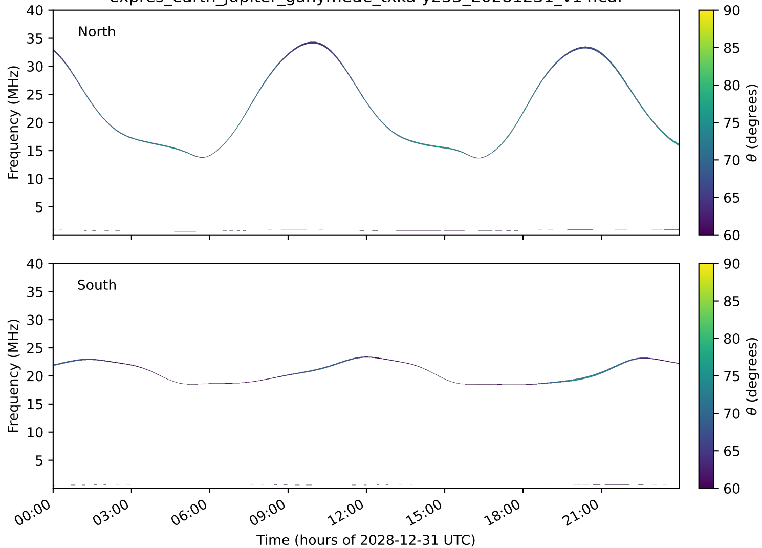
expres_earth_jupiter_ganymede_txka-y235_20281231_v14.cdf
