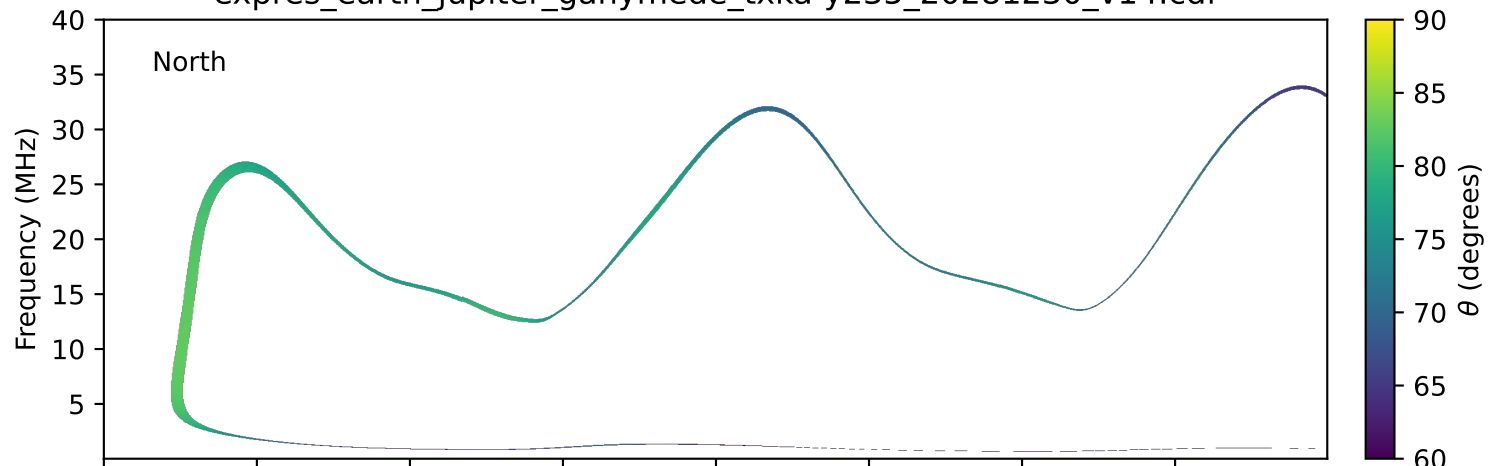
expres_earth_jupiter_ganymede_txka-y235_20281230_v14.cdf
