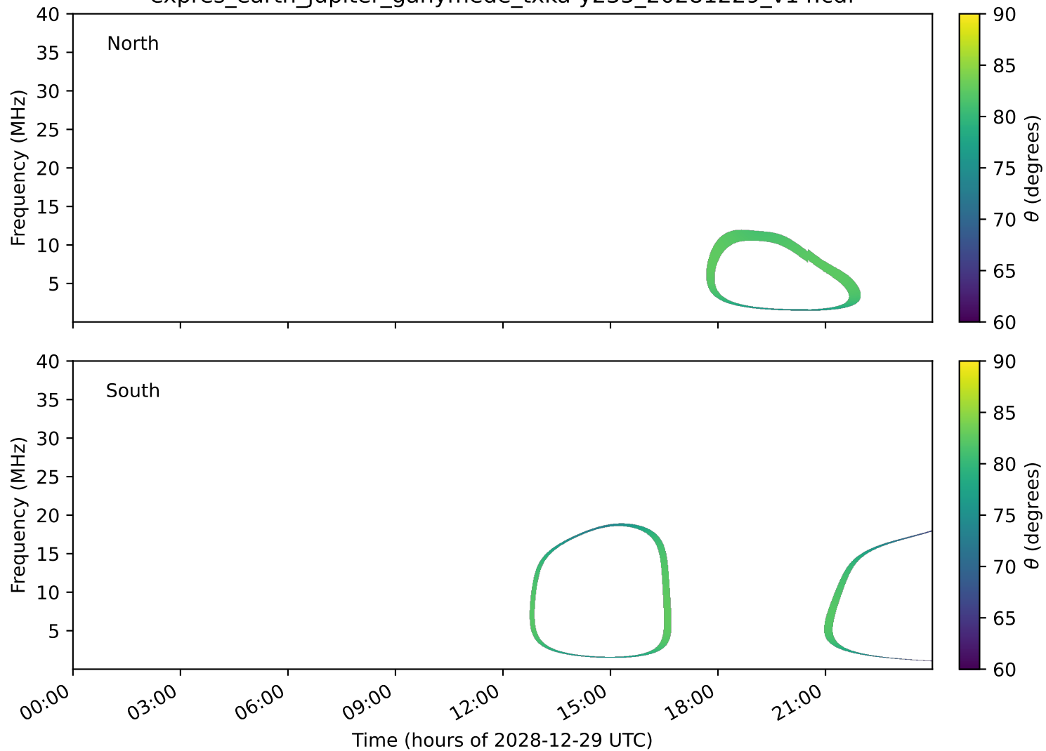
expres_earth_jupiter_ganymede_txka-y235_20281229_v14.cdf
