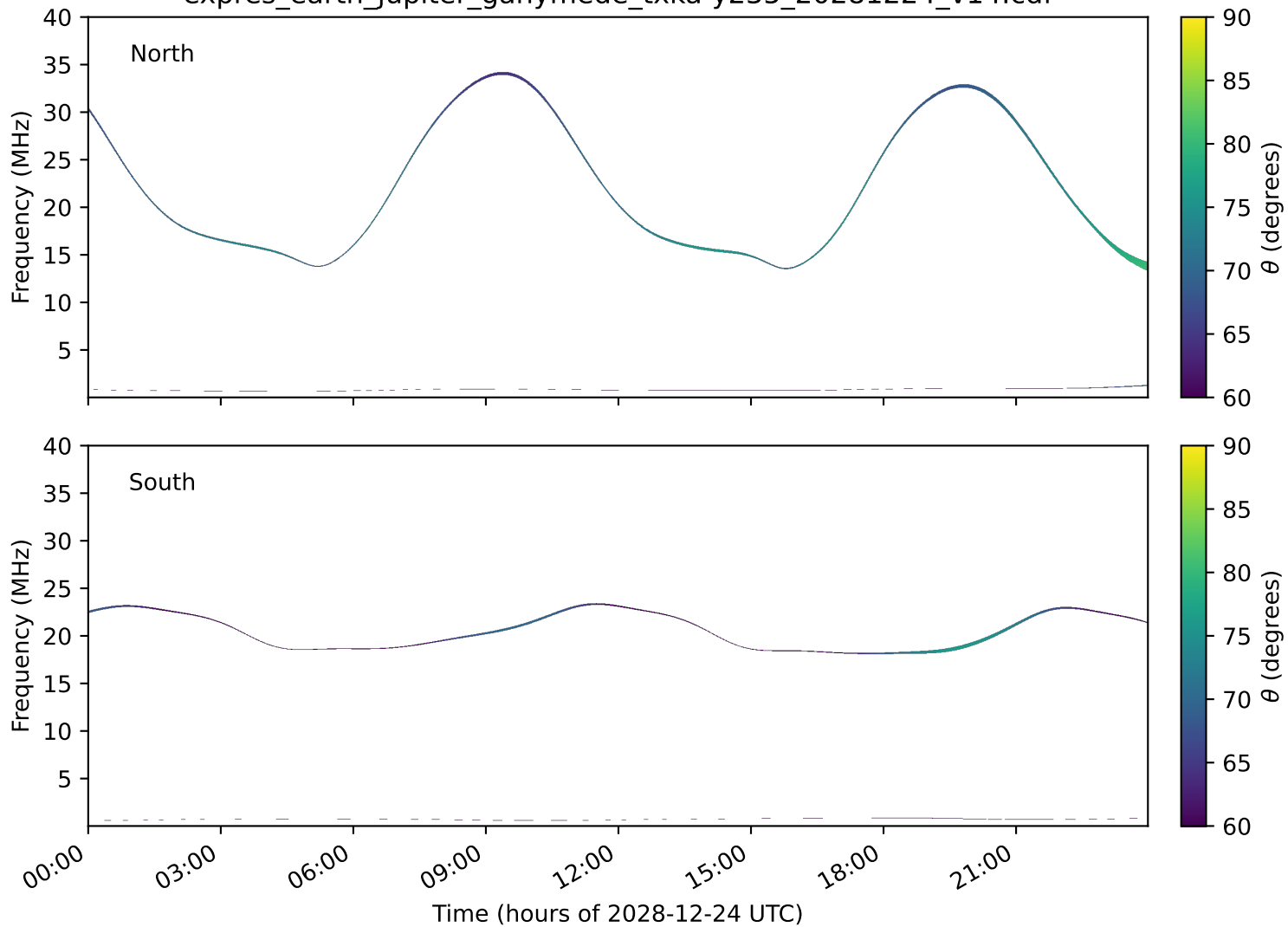
expres_earth_jupiter_ganymede_txka-y235_20281224_v14.cdf
