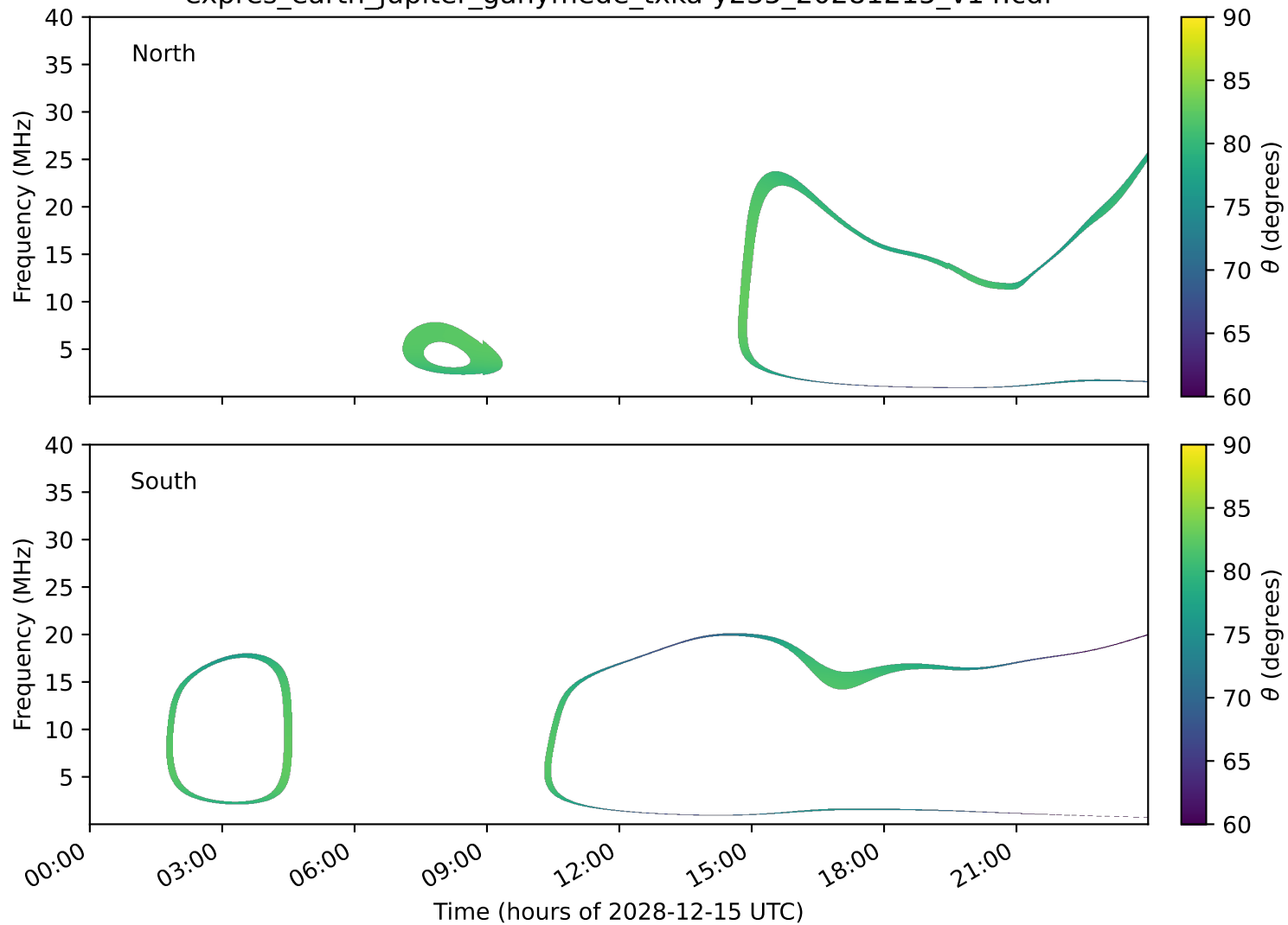
expres_earth_jupiter_ganymede_txka-y235_20281215_v14.cdf
