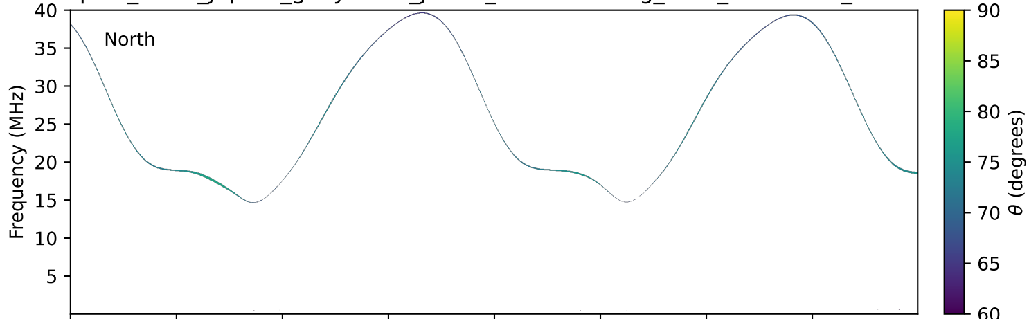
expres_earth_jupiter_ganymede_jrm33_lossc-wid1deg_3kev_20281231_v11.cdf
