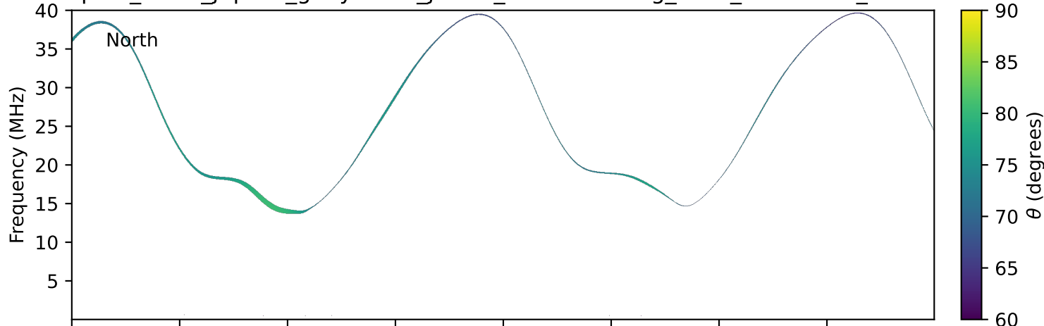
expres_earth_jupiter_ganymede_jrm33_lossc-wid1deg_3kev_20281209_v11.cdf
