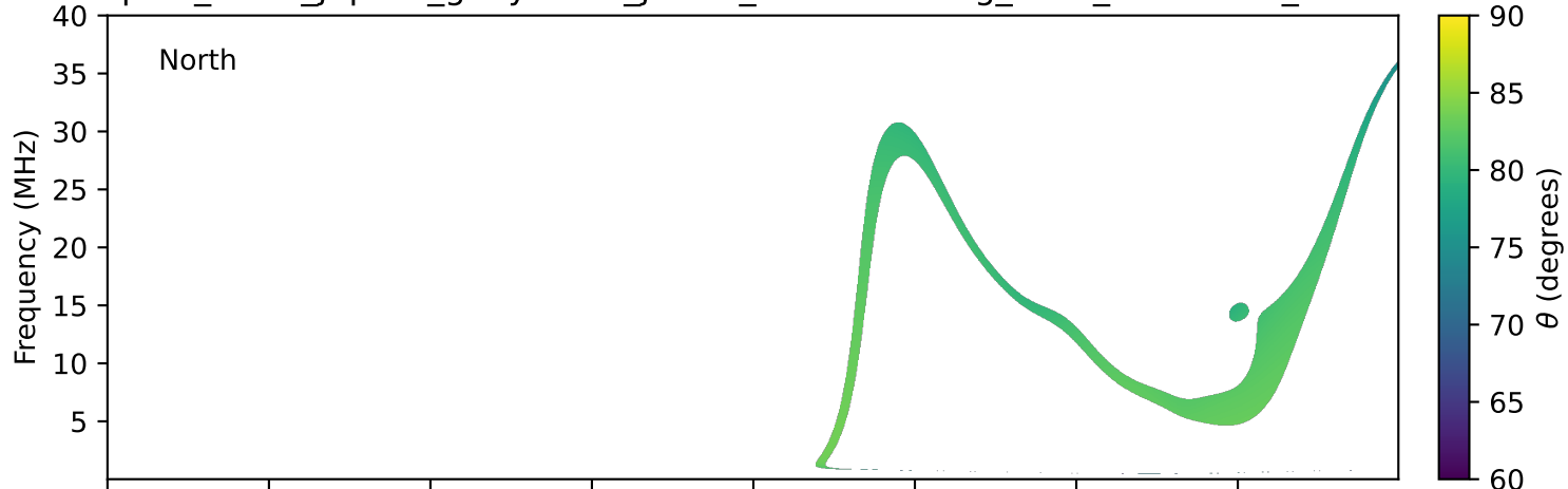
expres_earth_jupiter_ganymede_jrm33_lossc-wid1deg_3kev_20281208_v11.cdf
