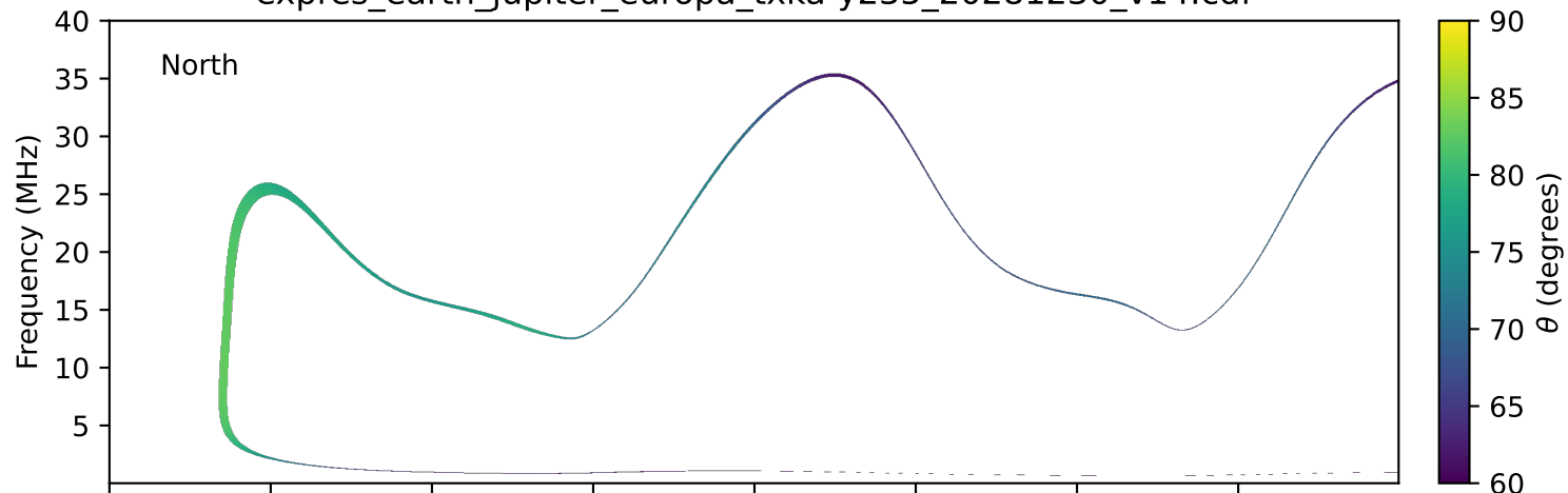
expres_earth_jupiter_europa_txka-y235_20281230_v14.cdf
