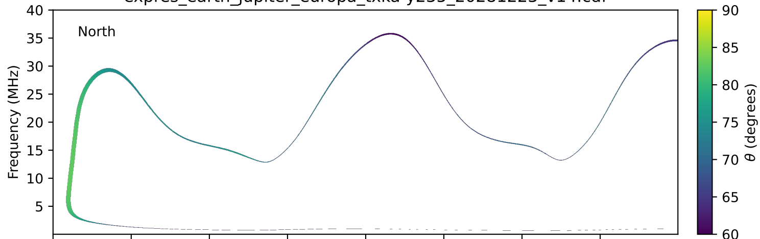
expres_earth_jupiter_europa_txka-y235_20281223_v14.cdf
