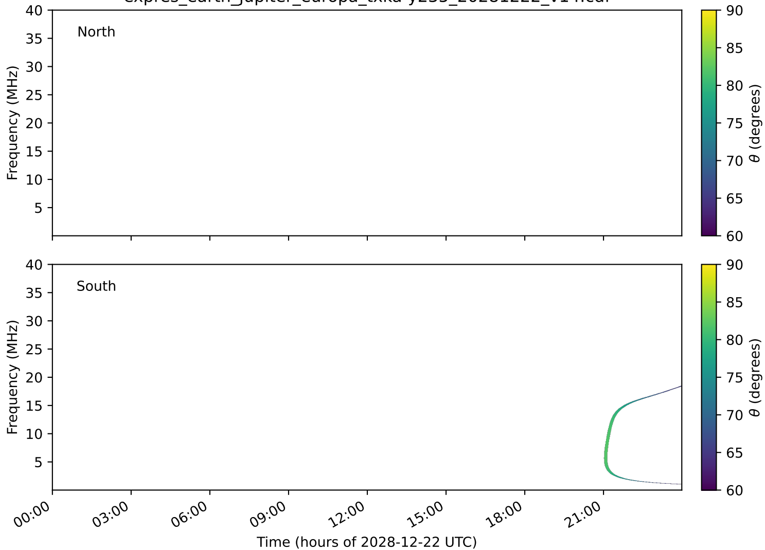
expres_earth_jupiter_europa_txka-y235_20281222_v14.cdf
