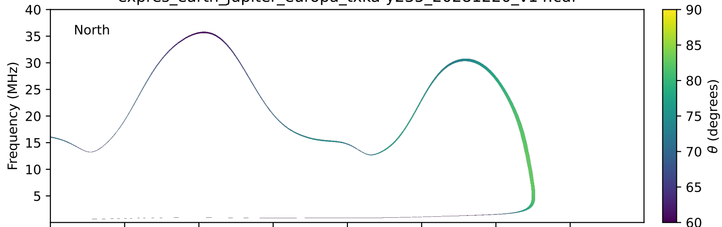
expres_earth_jupiter_europa_txka-y235_20281220_v14.cdf
