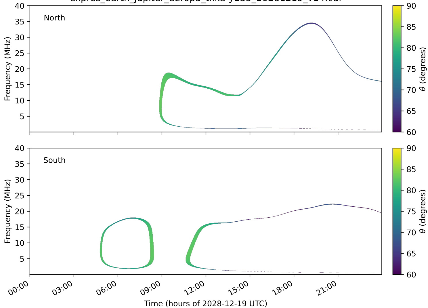
expres_earth_jupiter_europa_txka-y235_20281219_v14.cdf
