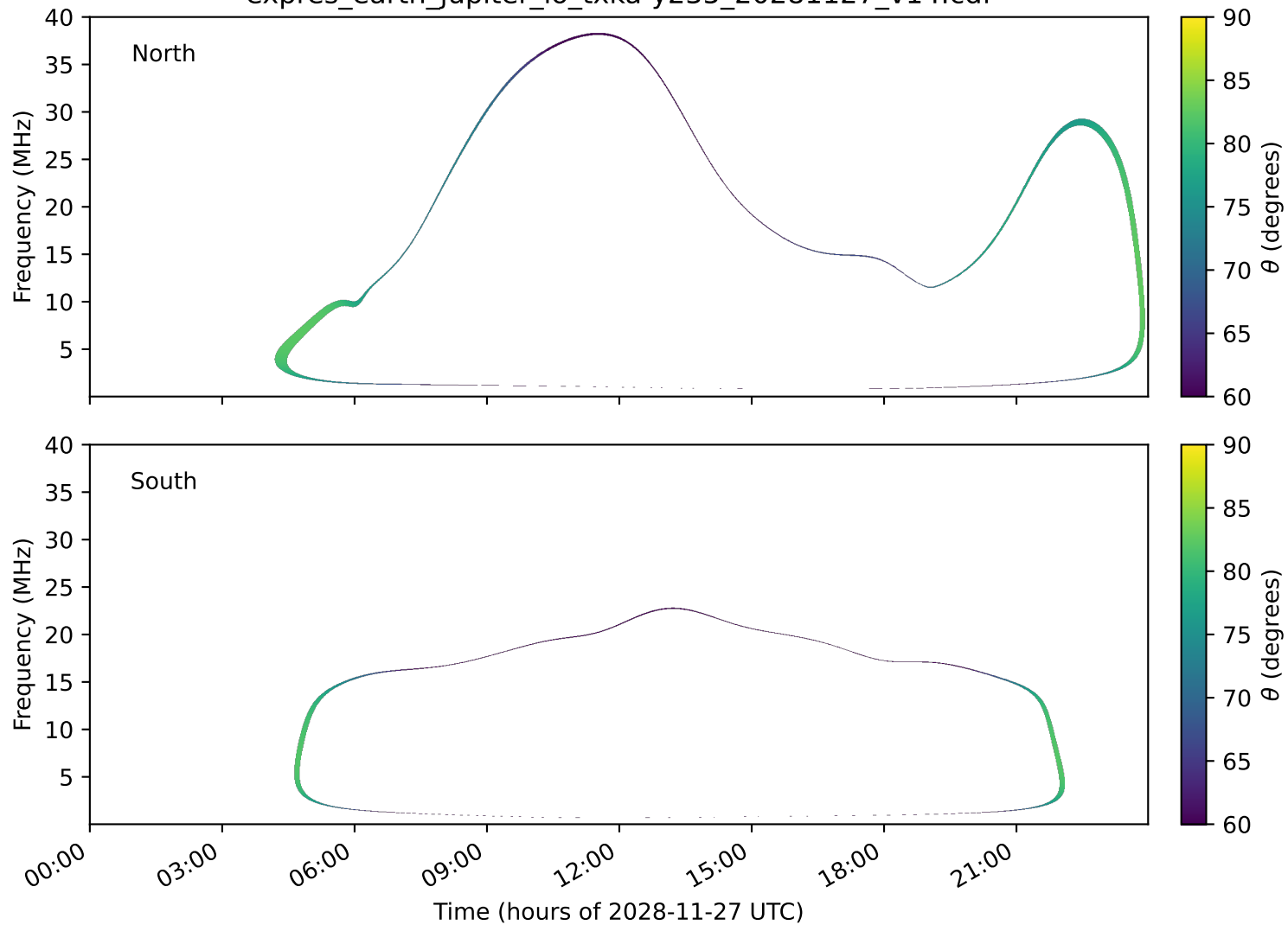
expres_earth_jupiter_io_txka-y235_20281127_v14.cdf
