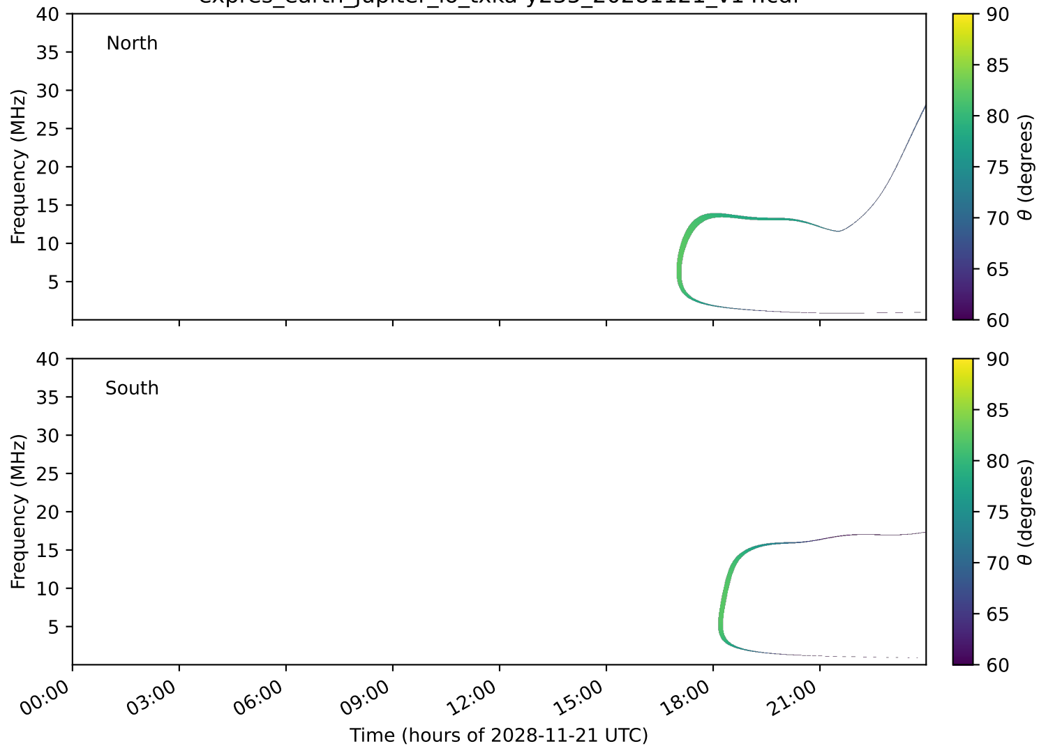
expres_earth_jupiter_io_txka-y235_20281121_v14.cdf
