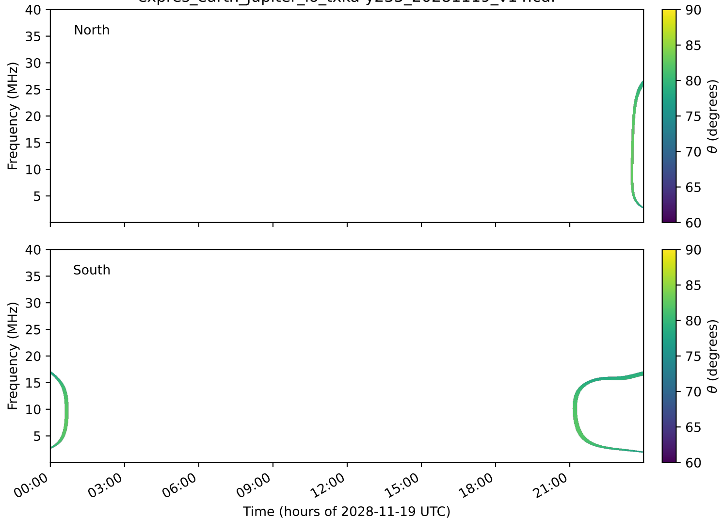
expres_earth_jupiter_io_txka-y235_20281119_v14.cdf
