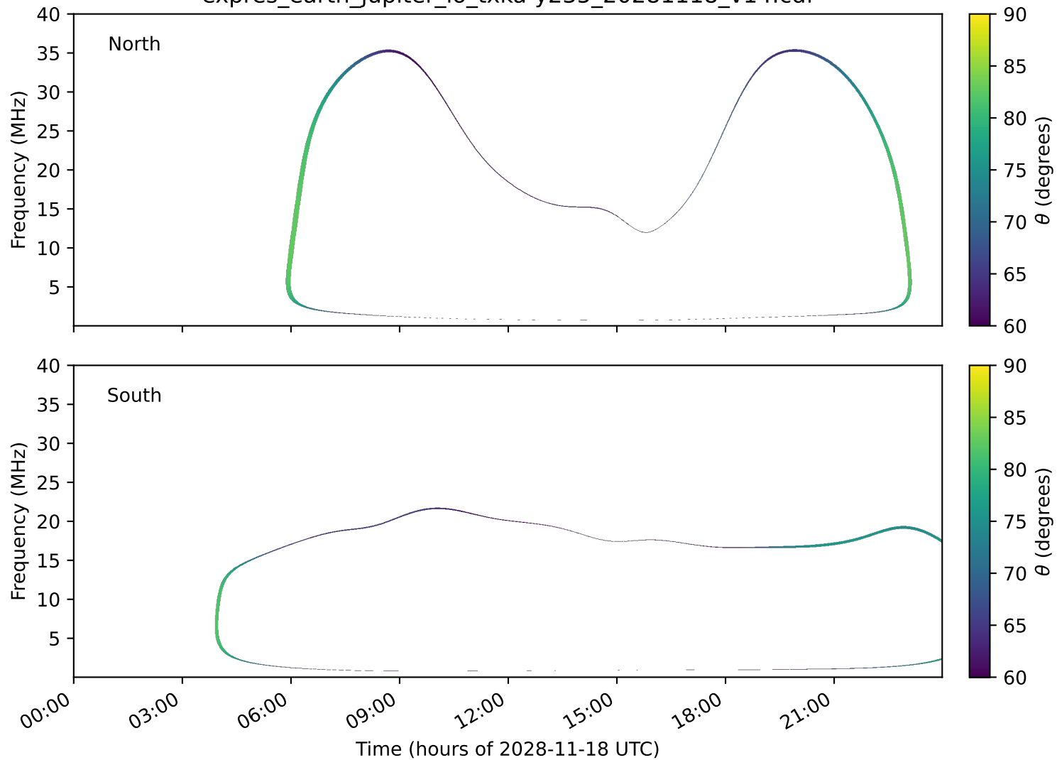
expres_earth_jupiter_io_txka-y235_20281118_v14.cdf
