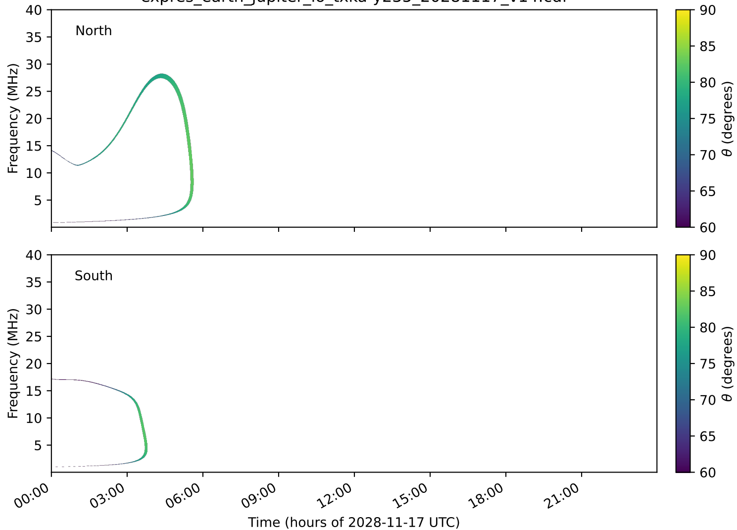
expres_earth_jupiter_io_txka-y235_20281117_v14.cdf
