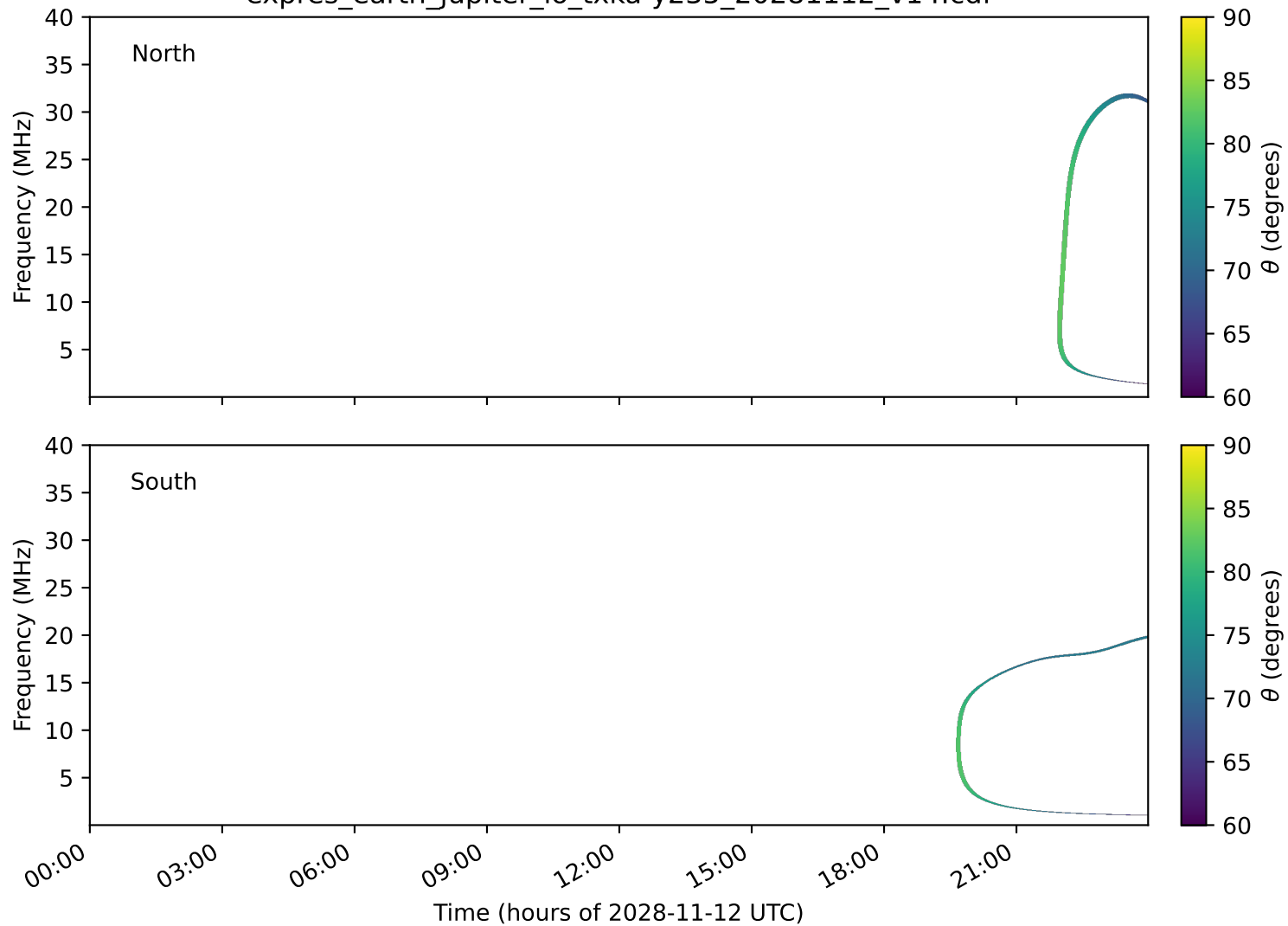
expres_earth_jupiter_io_txka-y235_20281112_v14.cdf
