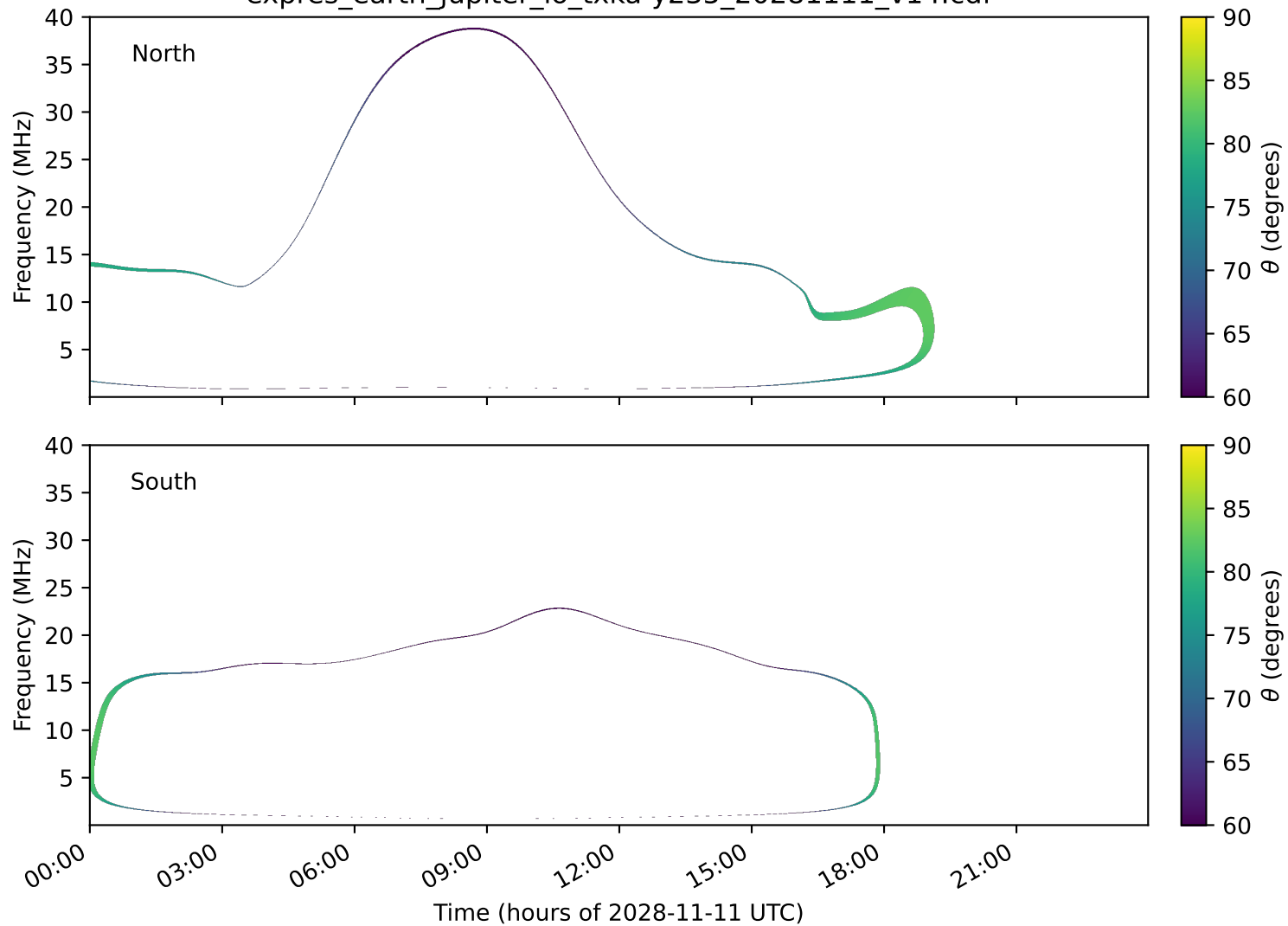
expres_earth_jupiter_io_txka-y235_20281111_v14.cdf
