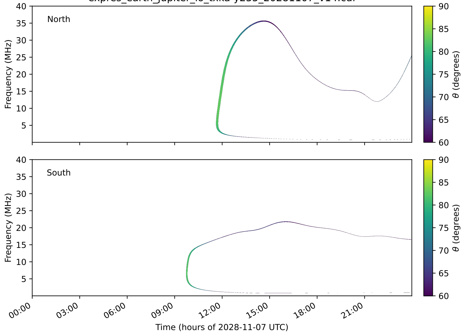
expres_earth_jupiter_io_txka-y235_20281107_v14.cdf
