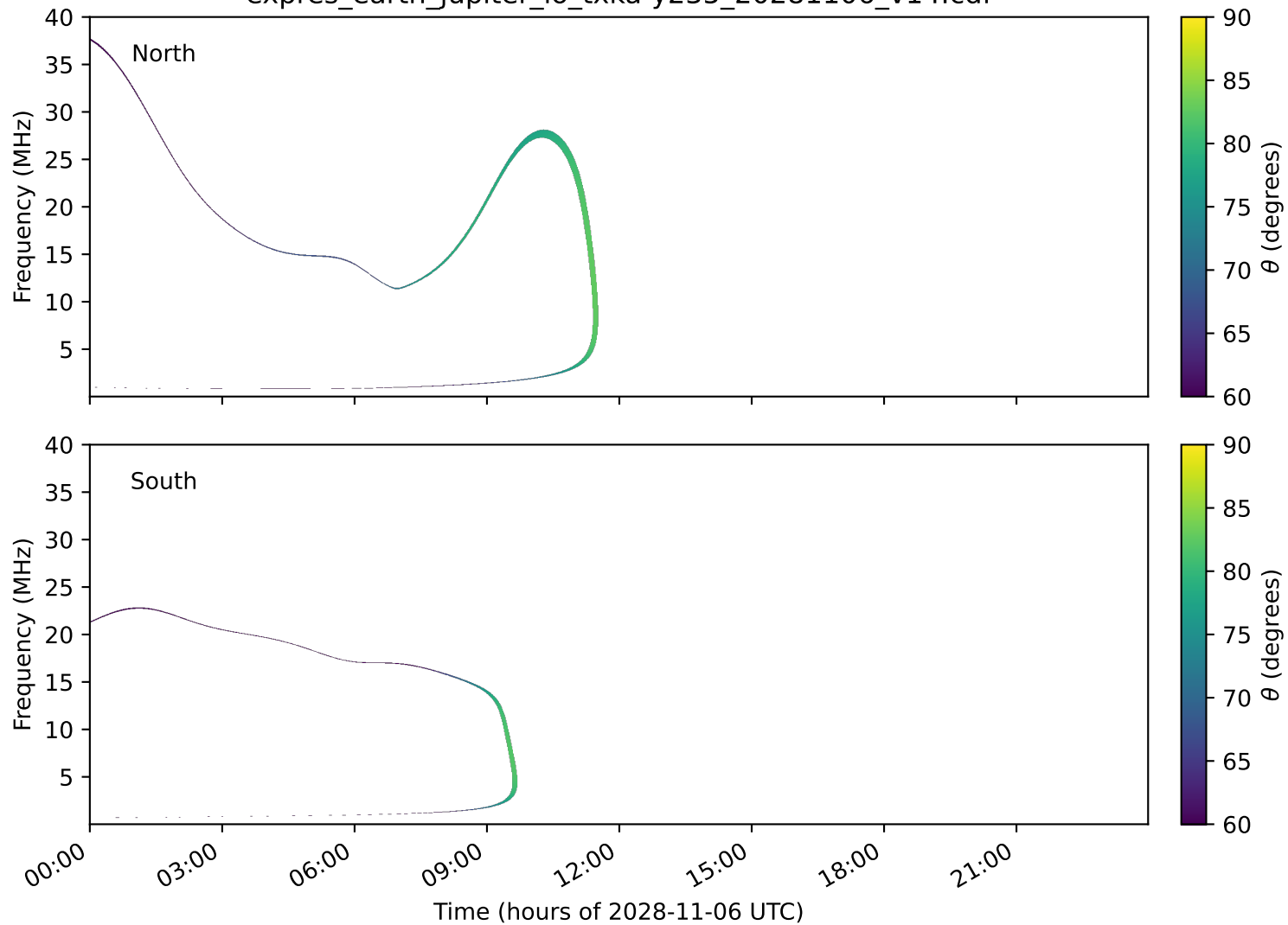
expres_earth_jupiter_io_txka-y235_20281106_v14.cdf
