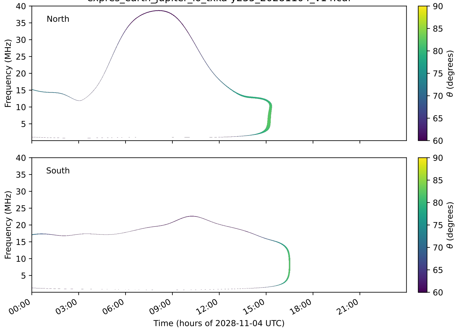
expres_earth_jupiter_io_txka-y235_20281104_v14.cdf
