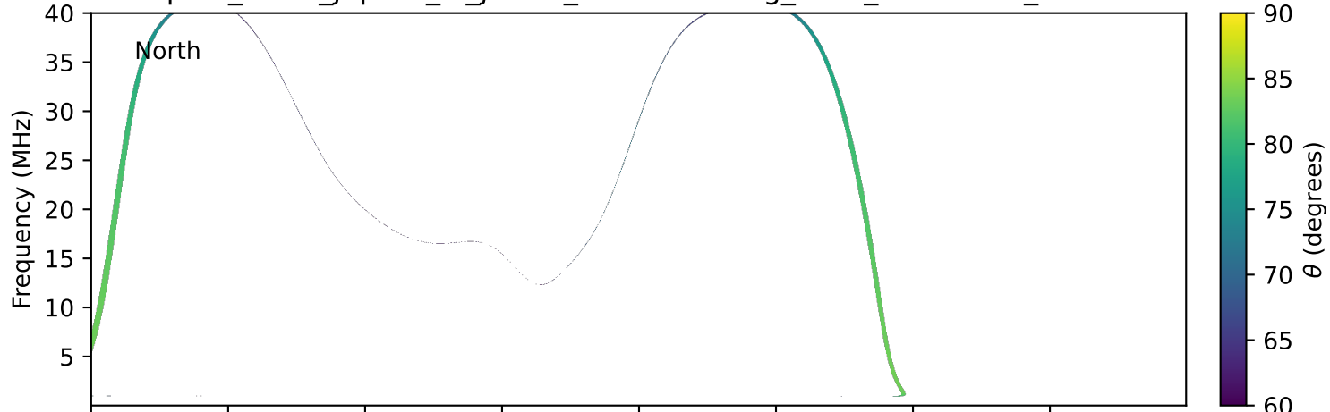
expres_earth_jupiter_io_jrm33_lossc-wid1deg_3kev_20281129_v11.cdf
