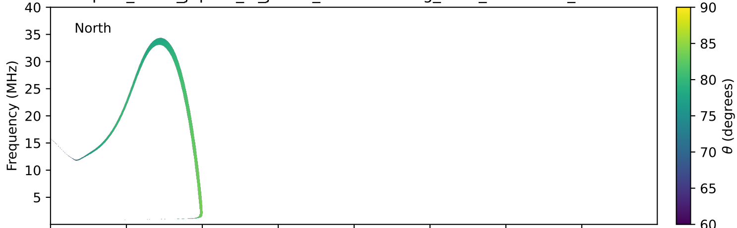
expres_earth_jupiter_io_jrm33_lossc-wid1deg_3kev_20281117_v11.cdf
