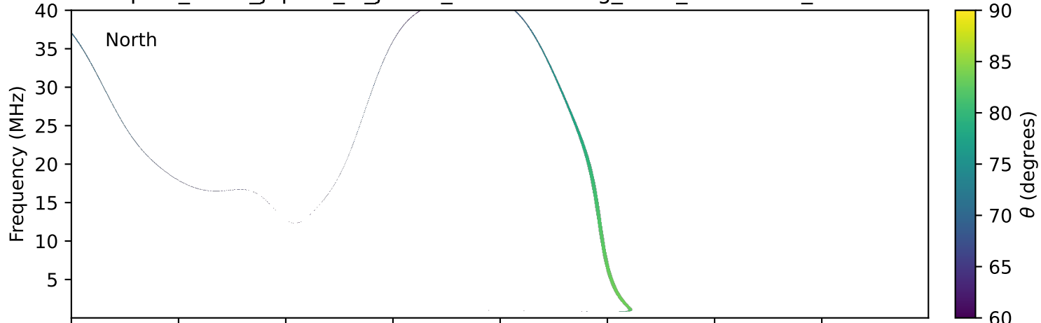
expres_earth_jupiter_io_jrm33_lossc-wid1deg_3kev_20281113_v11.cdf
